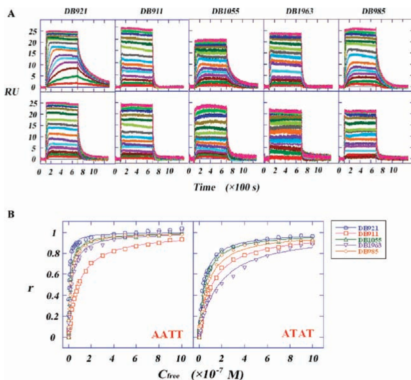
Figure 2. SPR binding affinity: (A) representative SPR sensorgrams for the interaction of selected compounds with AATT (upper panel) and ATAT (lower panel) DNA sequences. In all cases the compound concentrations from bottom to top are 0–1 \mu\text{M} . (B) Comparison of the SPR binding affinity for AATT and ATAT DNA sequences with different compounds. RU values from the steady-state region of SPR sensorgrams, such as those in (A), were converted to r ( r = \text{RU}/\text{RU}_{\text{max}} ) and are plotted against the unbound compound concentration (flow solution) for DB921 (circles), DB911 (squares), DB1055 (up triangle), DB1963 (down triangle), and DB985 (diamond) binding with AATT and ATAT DNA sequences. The lines are the best fit values to a single site interaction model as described in the text.
