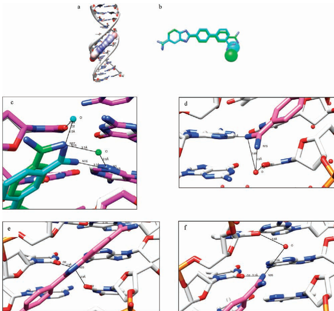
Figure 6. X-ray crystallography: (a) The crystal structure of the DB1055-d(CGCGAATTCGCG) 2 complex, with the DNA in cartoon ribbon representation and the ligand shown bound in the minor groove as a solvent-accessible surface colored according to B factor values. (b) Overlay of the crystal structure positions of DB1055 (blue sticks) and DB921 (green sticks), together with the associated water molecule, colored in the same way. (c) Detailed view of the meta and para amidinium ends of DB1055 and DB921, using the same color representations as in Figure 5, showing H-bond interactions with the DNA and water molecules. (d–f) Views of the H-bonding between the three regions of DB1055 and the minor groove substituents; (d) shows the meta amidinium group, (e) shows the central imidazole group, and (f) shows the benzimidazole amidinium group.
