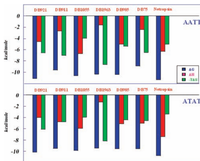
Figure 4. Comparison of binding thermodynamics values for selected compound with AATT and ATAT DNA sequences at 25 ^\circ\text{C} .
