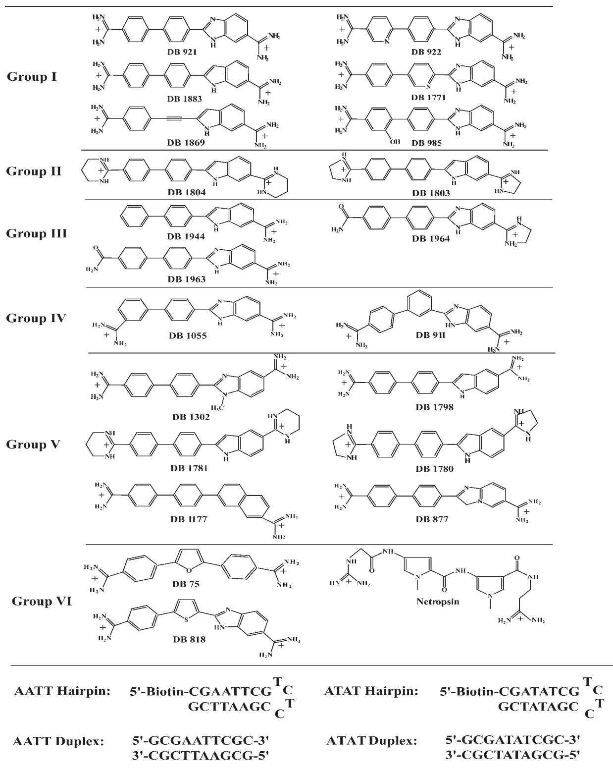
Figure 1. Structure of the compounds and the DNA sequences used in this study. The DNA hairpins were used in SPR with biotin (as shown) and in ITC without biotin.
