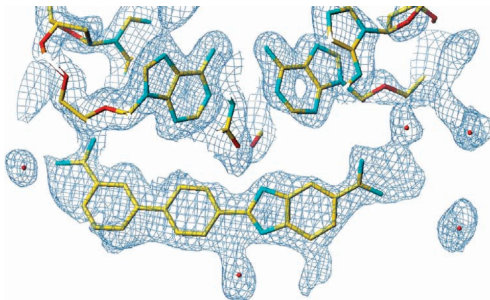
Figure 7. An electron density contour at 1.3\sigma of a 2F_o - F_c map with the DB1055 structure overlaid in the DNA minor groove.
