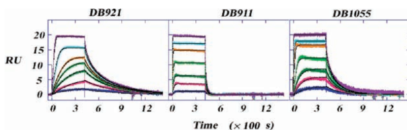
Figure 3. SPR sensorgrams to evaluate the kinetics of the interactions of DB921, DB911, and DB1055 with the AATT DNA sequence in MES20 buffer at a 50 \mu\text{L}/\text{min} flow rate are shown. The black lines are best fit curves determined by global kinetic fitting. The concentrations from bottom to top are: 0.001, 0.003, 0.006, 0.012, 0.03, and 0.065 \mu\text{M} for DB921; 0.004, 0.015, 0.03, 0.08, 0.15, 0.9 \mu\text{M} for DB911; and 0.003, 0.009, 0.015, 0.045, 0.1, 0.15, 0.75 \mu\text{M} for DB1055, respectively.
